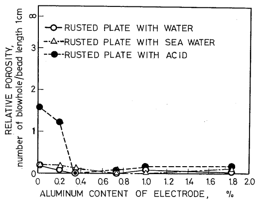
Fig. 9 Effect of aluminum content of electrode wire on the porosity of weld metal of rusted steel plates.
