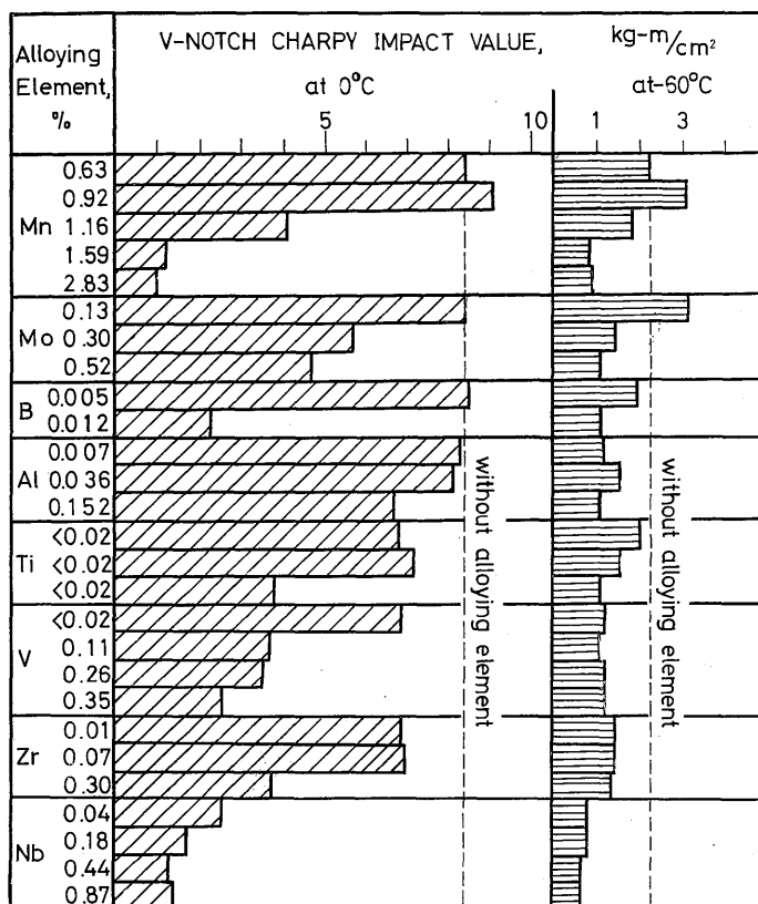
Fig. 1 Effect of alloying elements on notch toughness of weld metal of 2½% nickel steel.
