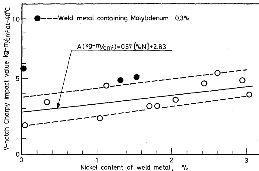
Fig. 2 Effect of nickel content on notch toughness of weld metal.
