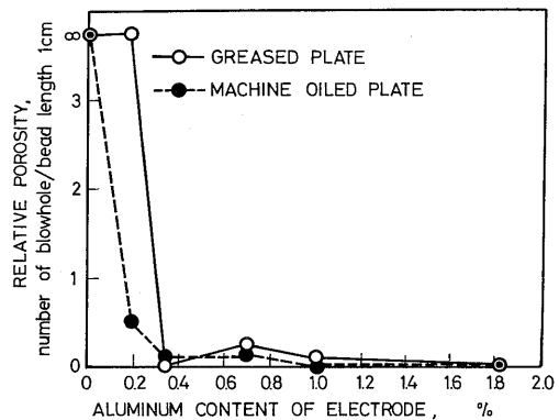
Fig. 11 Effect of aluminum content of electrode wire on the porosity of weld metal of greased and oiled steel plates.
