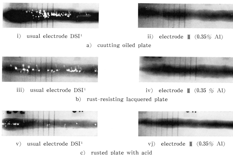
Photo. 2 Effect of aluminum content on the porosity of weld metal of oiled a), lacquered b) and rusted c) steel plate.
