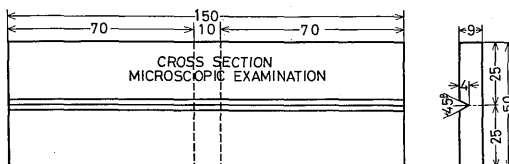
Fig. 8 Bead-on-plate test pieces with groove, unit: mm.
