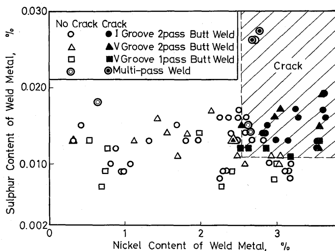
Fig. 4 Effect of nickel and sulphur contents on the hot crack in weld metal.
