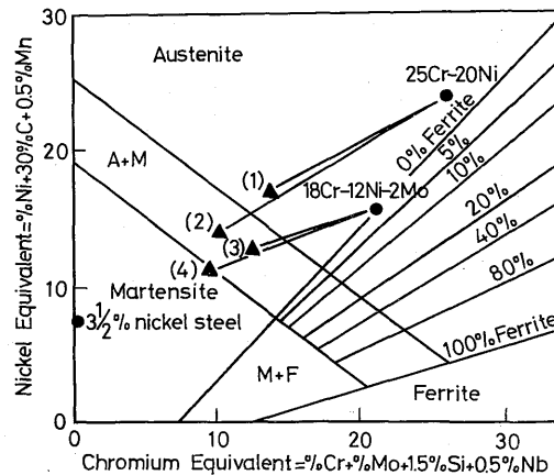
Fig. 7 Constitution diagram for stainless steel weld metal. Remarks: Base metal; 3\frac{1}{2}\% nickel steel
