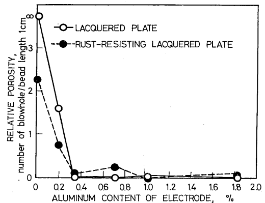
Fig. 10 Effect of aluminum content of electrode wire on the porosity of weld metal of lacquered steel plates.
