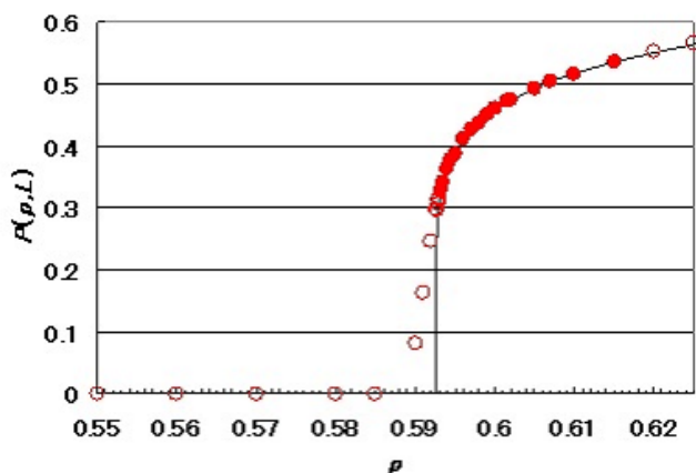
Fig.1 The mean value of percolation fraction P(p, L) is shown by circles. The solid line is obtained by using the critical parameter of Table 1.
