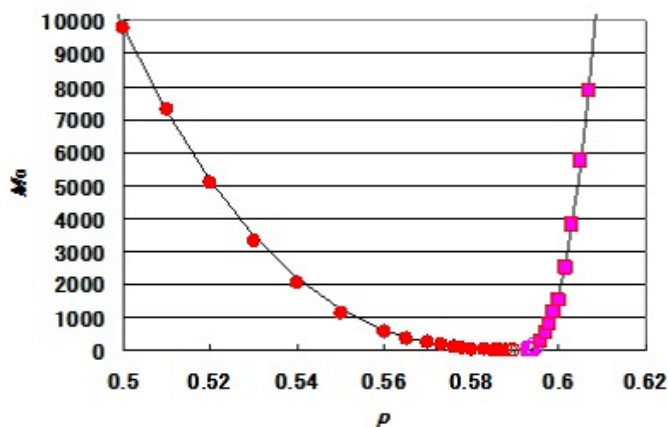
Fig.3 The total number of finite clusters M_0 is plotted against p by circles (below p_c ) and by squares (above p_c ). The solid line is obtained by using the critical parameters of Table 1.
