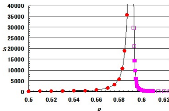
Fig.5 The mean cluster size S is plotted against p by circles (below p_c ) and by squares (above p_c ). The solid line is obtained by using the critical parameters of Table 1.
