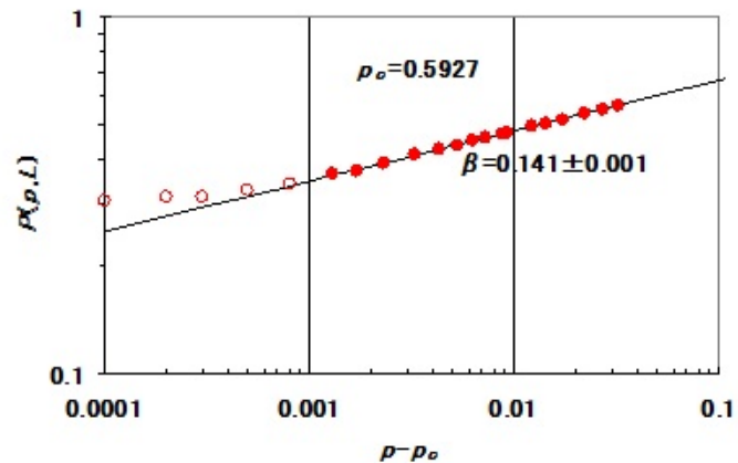
Fig.2 (b) The percolation fraction \log(P(p, L)) is plotted against \log(p - p_c) . When the adjustable value of p_c is assumed to be 0.5927, the critical exponent \beta becomes 0.141.
