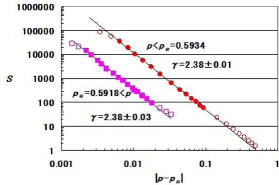
Fig.6 (b) The mean cluster size \log(S) is plotted against \log(|p - p_c|) . We try to find the best straight line by tuning p_c , below and above p_c , respectively. From the slope we have obtained \gamma = 2.38 both below and above p_c .
