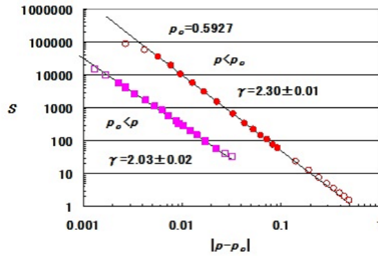
Fig.6 (a) The mean cluster size \log(S) is plotted against \log(|p - p_c|) . When the adjustable value of p_c is assumed to be 0.5927, from the slope we have obtained \gamma = 2.30 (below p_c ) and \gamma = 2.03 (above p_c ).
