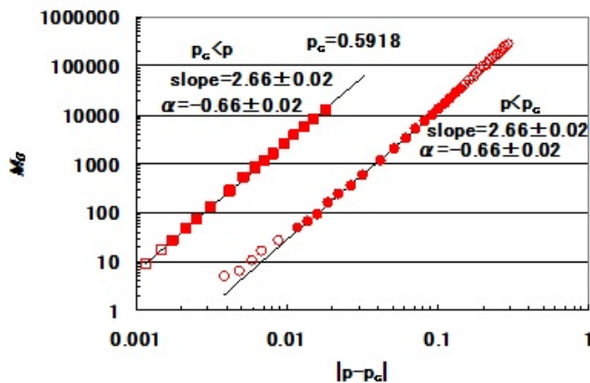
Fig.4 (b) The total number of finite clusters \log(M_0) is plotted against \log(|p - p_c|) . We try to find the best straight line by tuning p_c , below and above p_c , respectively. From the slope we have obtained \alpha = -0.66 both below and above p_c .
