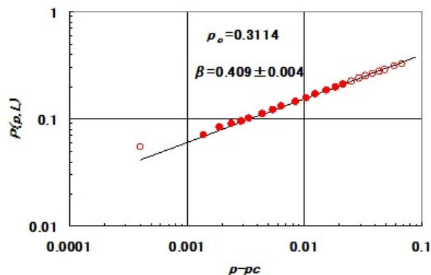
Fig.7 The percolation fraction \log(P(p, L)) is plotted against \log(p - p_c) . We try to find the best straight line by tuning p_c . The value of p_c obtained is 0.3114 and the slope is obtained \beta = 0.409 .
