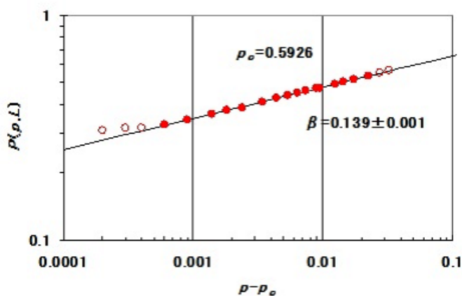
Fig.2 (a) The percolation fraction \log(P(p, L)) is plotted against \log(p - p_c) . We try to find the best straight line by tuning p_c . The value of p_c obtained is 0.5926 and the slope \beta = 0.139 is obtained.
