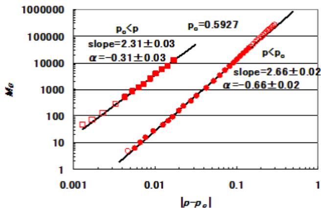
Fig.4 (a) The total number of finite clusters \log(M_0) is plotted against \log(|p - p_c|) . When the adjustable p_c is assumed to be 0.5927, from the slope we have obtained \alpha = -0.66 (below p_c ) and \alpha = -0.31 (above p_c ).
