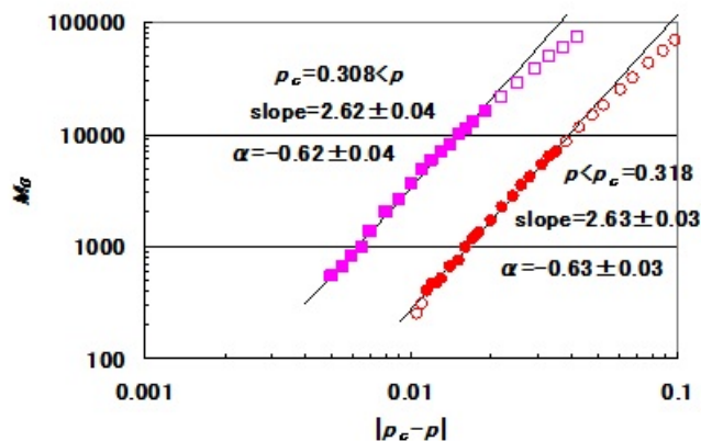
Fig.8 The total number of finite clusters \log(M_0) is plotted against \log(|p - p_c|) . We try to find the best straight line by tuning p_c , below and above p_c , respectively. From the slope we have obtained \alpha = -0.63 (below p_c ) and \alpha = -0.62 (above p_c ).
