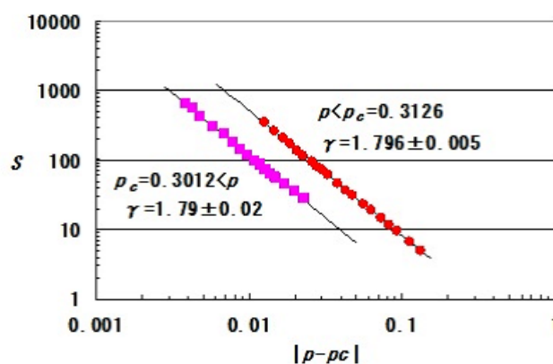
Fig.9 The mean cluster size \log(S) is plotted against \log(|p - p_c|) . We try to find the best straight line by tuning p_c , below and above p_c , respectively. From the slope we have obtained \gamma = 1.79 both below and above p_c .
